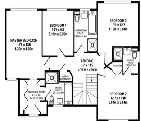
1ST FLOOR APPROX. FLOOR AREA 849 SQ.M. (914 SQ.FT.)
